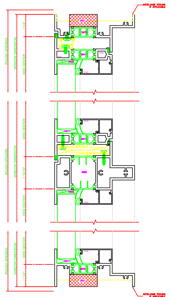
547 MEETING RAIL SERIES: 450X C.O./FIXED BUTT HINGE
