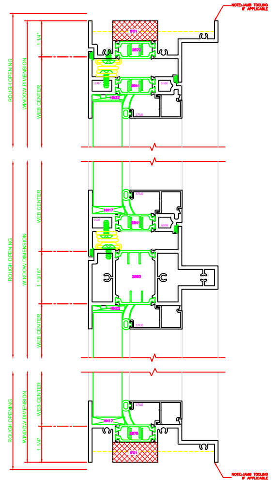
546 MEETING RAIL SERIES: 450X C.O./FIXED 4-BAR ARMS
